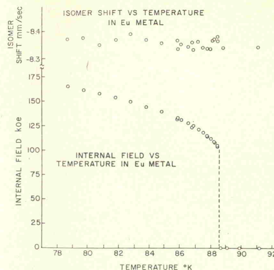
FIG. 3. (a) Observed internal fields plotted as a function of temperature. Note the sudden drop of the field at T_i . The ( 1\sigma ) error flags are about the size of the points. (b) Observed isomer shifts as a function of temperature. Note that there is no substantial discontinuity at T_i . Isomer-shift values are relative to an \text{Eu}_2\text{O}_3 absorber at 78°K.
